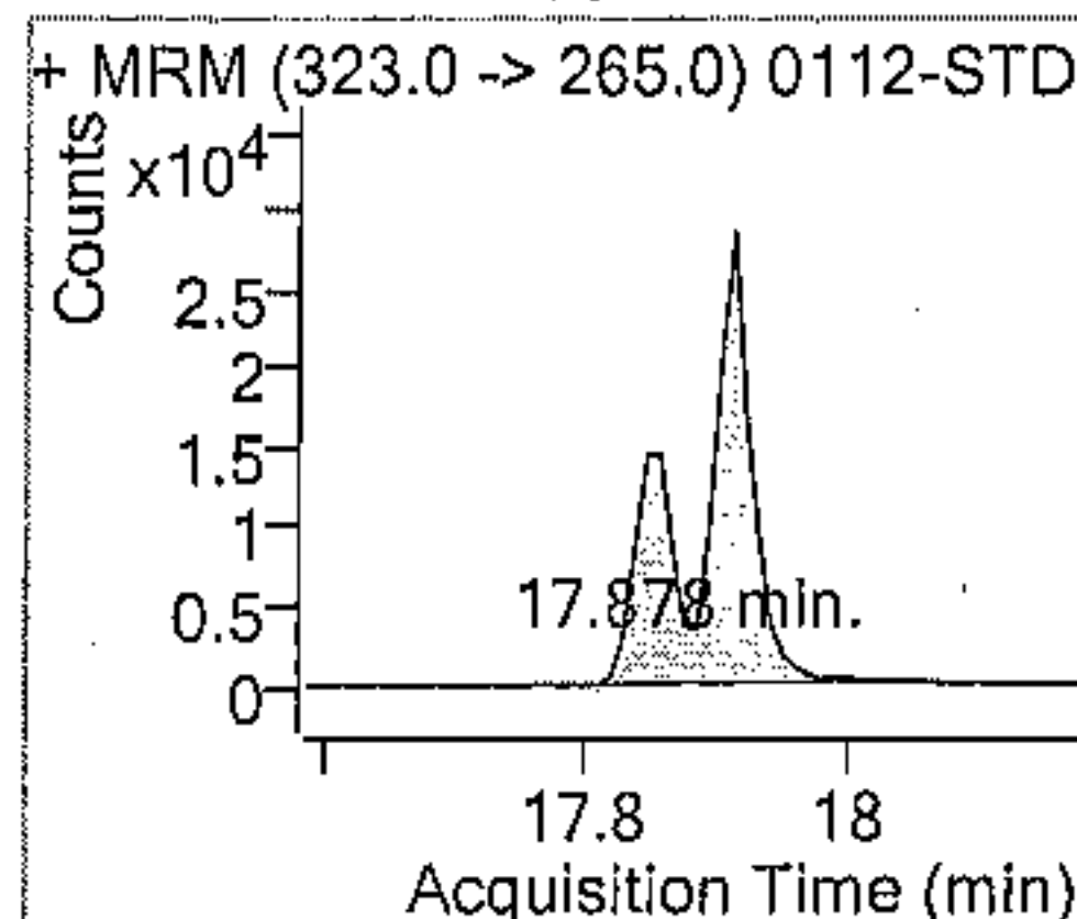
Procymidone 撲滅
