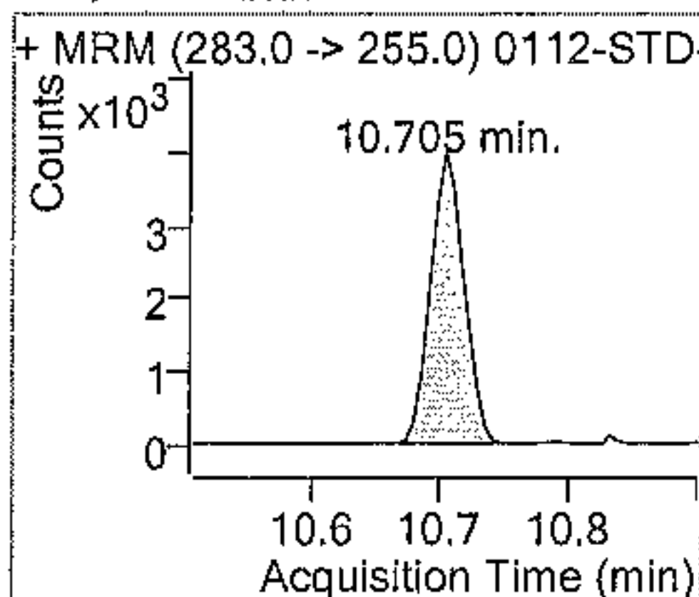
Procymidone 撲滅
